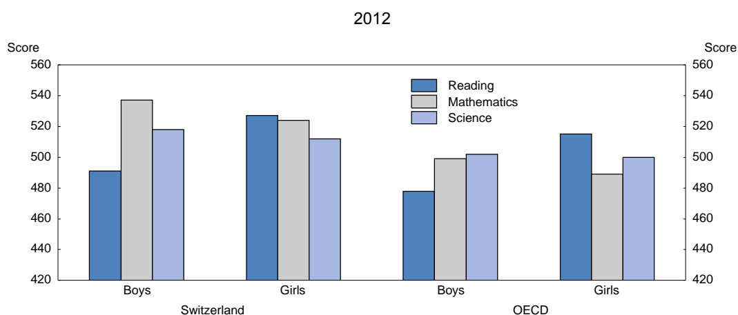
Figure 9. PISA scores
