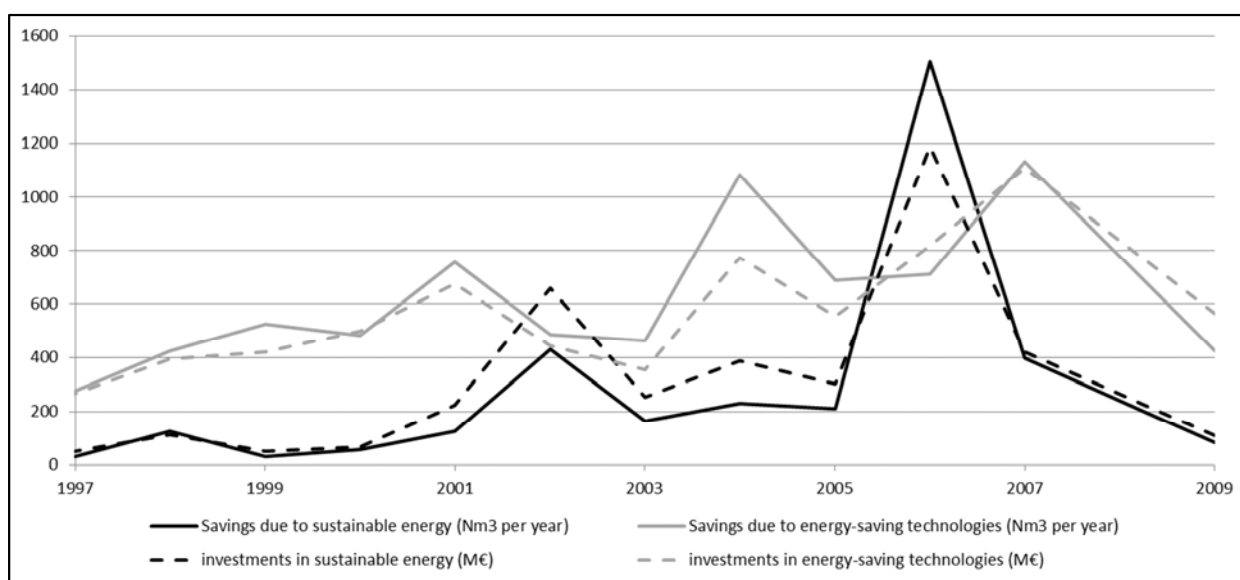
Figure 6. Energy savings for investments in sustainable energy and energy-saving technologies Million EUR and Nm 3
