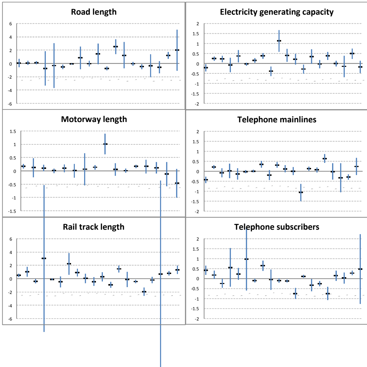
Figure 1. Infrastructure coefficient estimates from growth regressions
