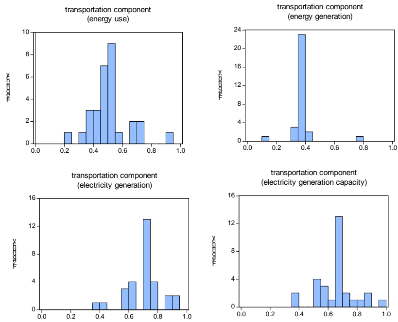
Figure A.1. Distribution of inclusion probability, 1 st principal component 10-year averages
