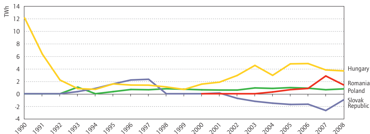
Ukraine net electricity trade with countries subject to the EU ETS (1990-2008)
