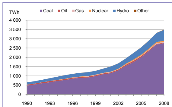
Figure 2 Generation mix in power sector
