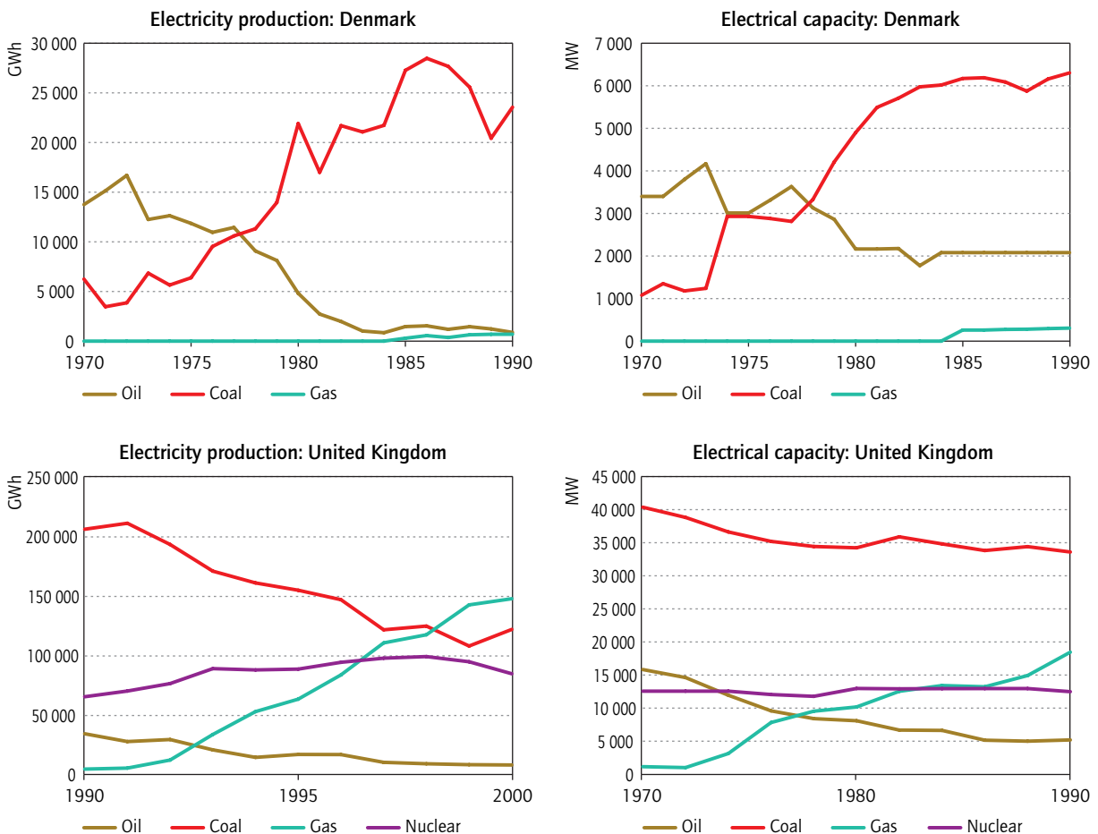
Figure 2 Historical electricity production and electrical capacity by fuel in Denmark and the United Kingdom
