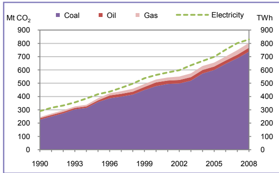
CO 2 emissions by fuel in electricity generation
