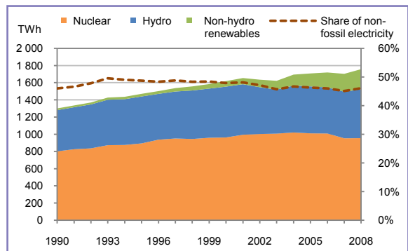
Figure 4 Electricity generation by non-fossil fuels
