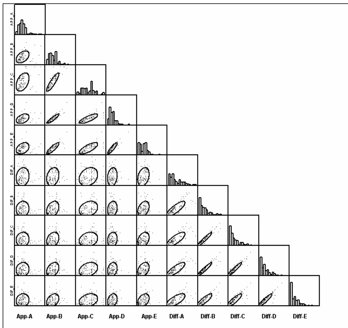
Figure 1: Scatter-plot matrix of applied tariffs and difference
