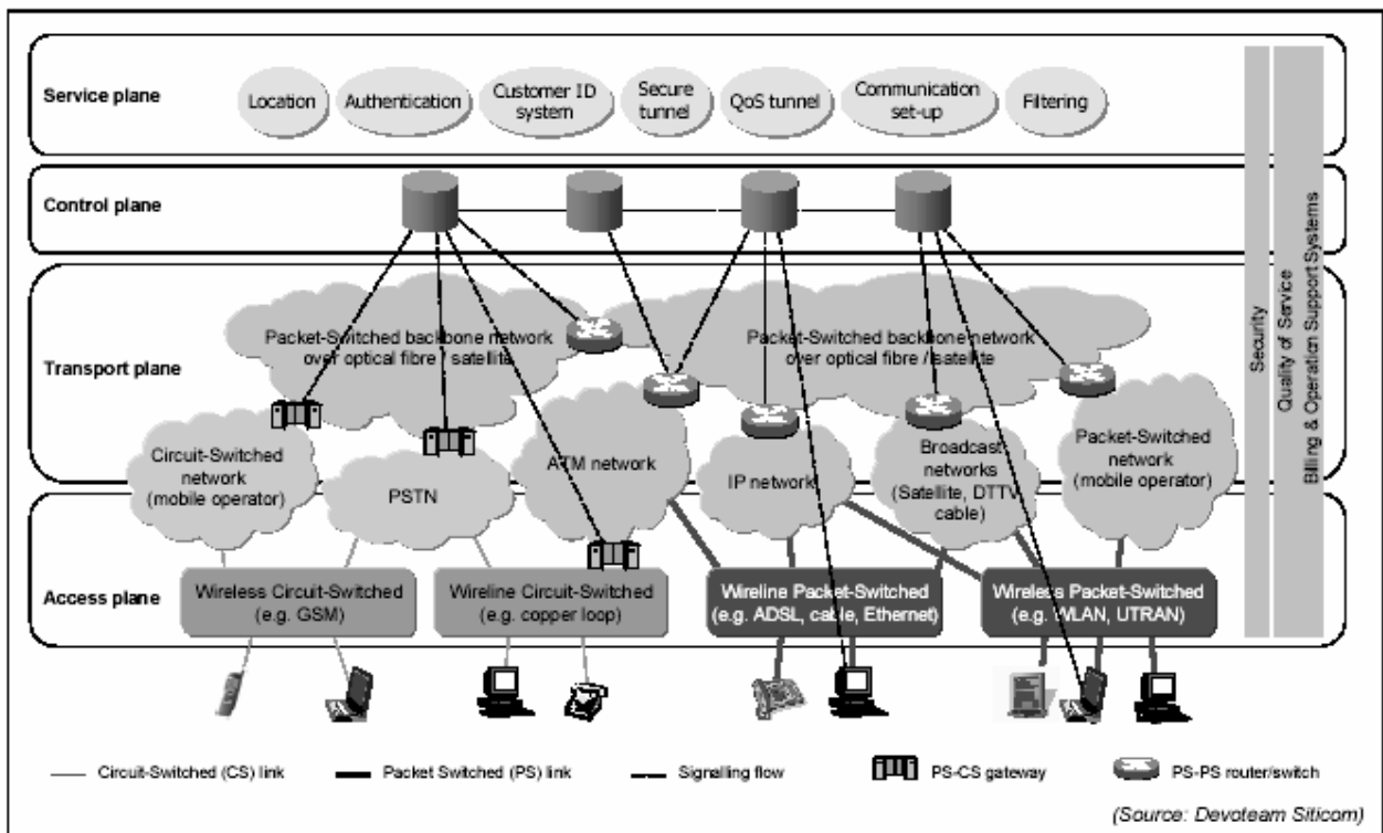
Figure 1: The architecture of NGN
