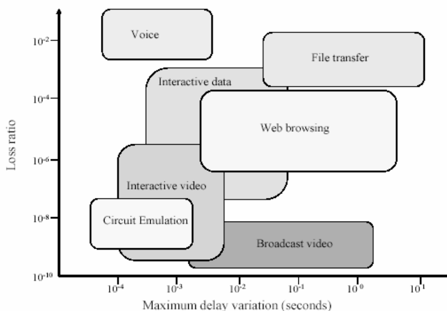
Figure 4: Application specific loss and delay variation in QoS requirements
