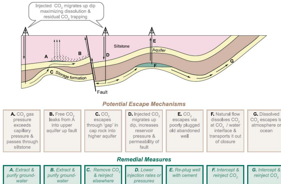
Figure 6: Potential leakage routes and remediation techniques for CO 2 injected into saline formations
