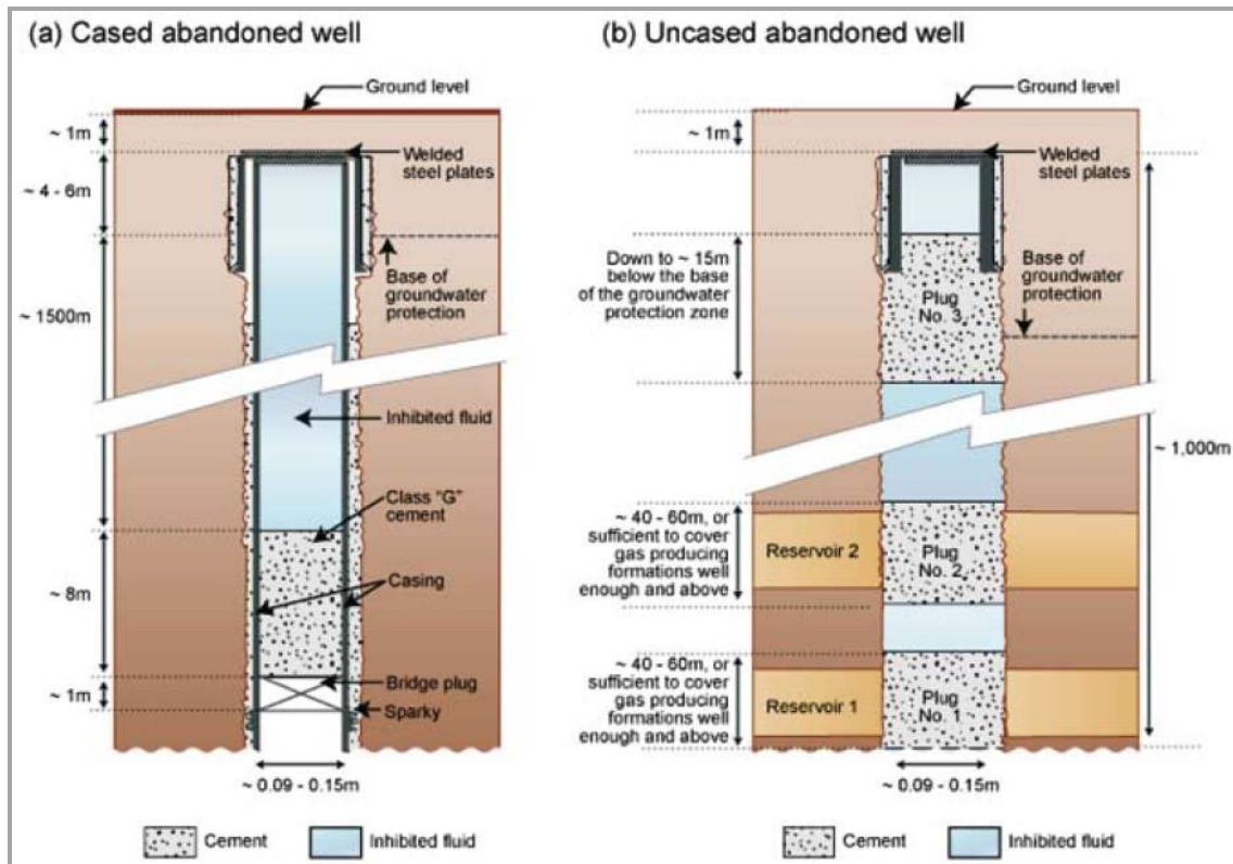
Figure 8: Example of how cased and uncased wells are abandoned today
