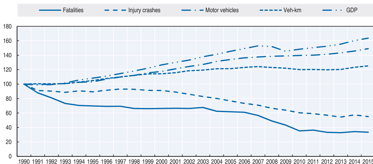
Figure 39.1. Road safety, traffic and GDP trends index 1990 = 100
