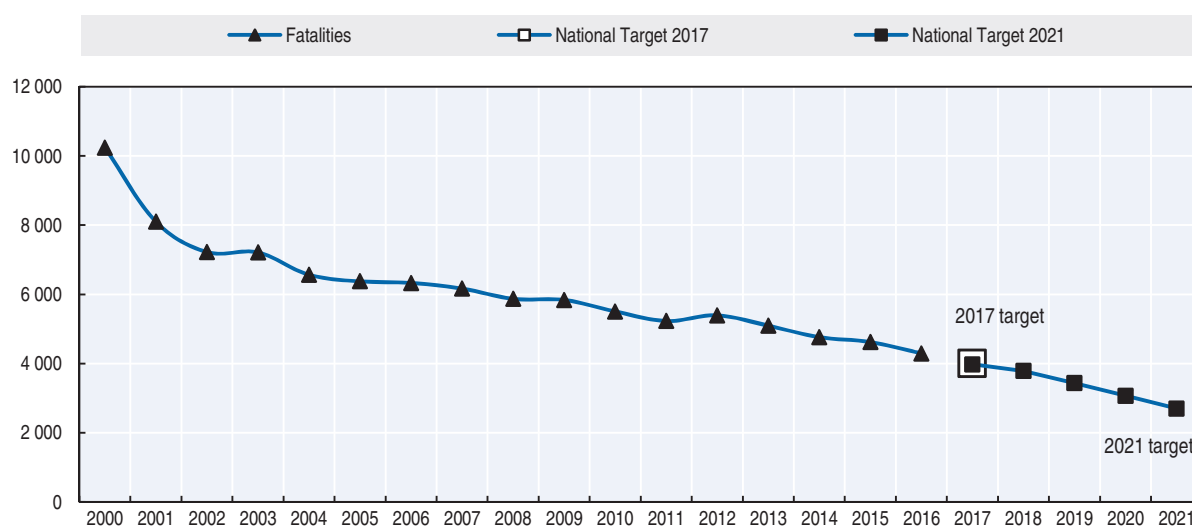
Figure 21.7. Trends in road fatalities towards national target
