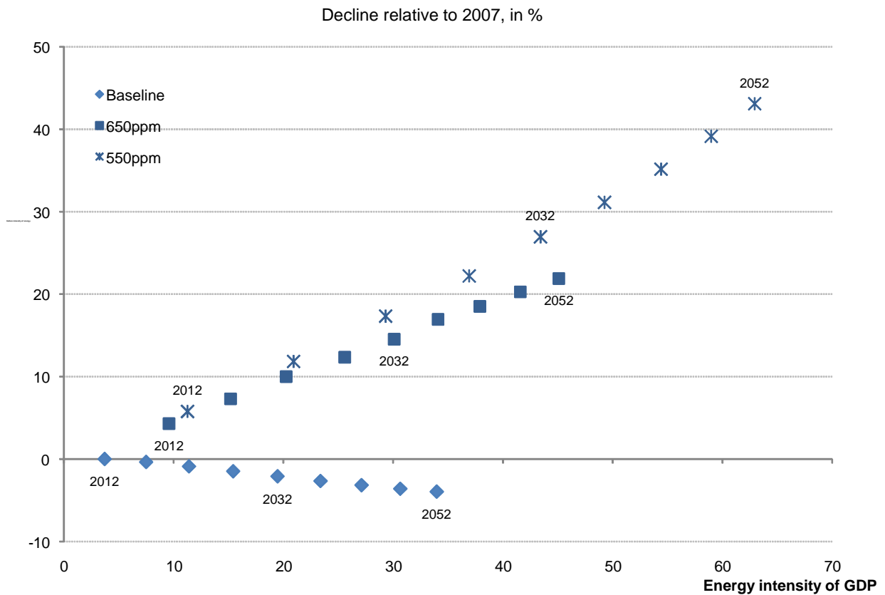
Figure 2. World energy intensity and carbon intensity trajectories under alternative carbon price paths 1
