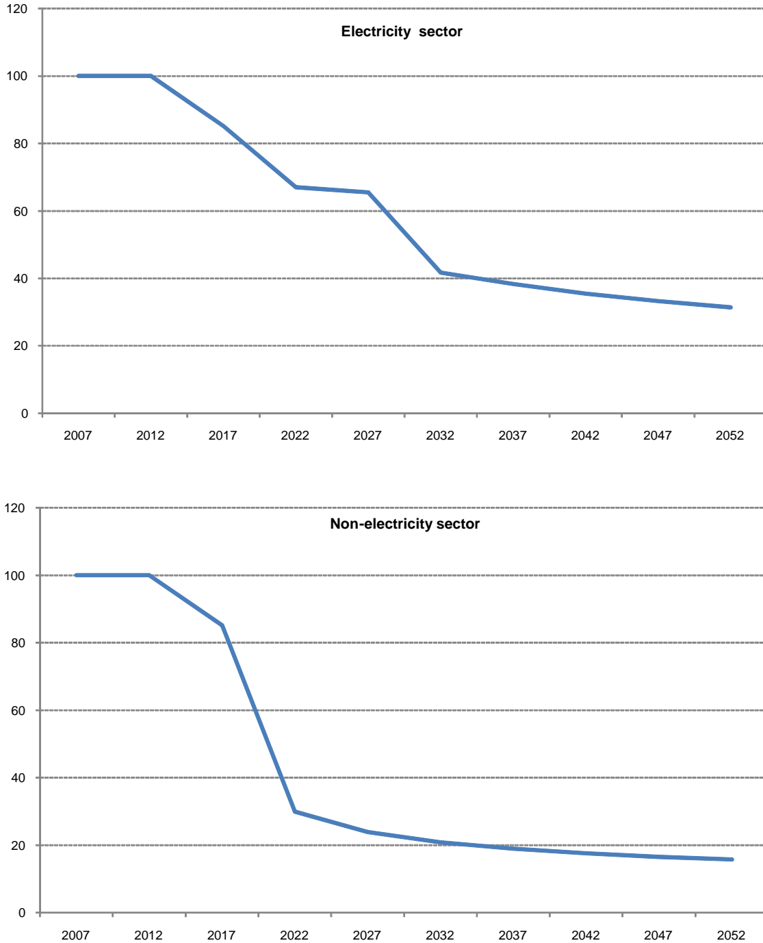
Figure 9. Simulated investment costs of the backstop technologies, 550ppm GHG concentration stabilisation scenario 1
