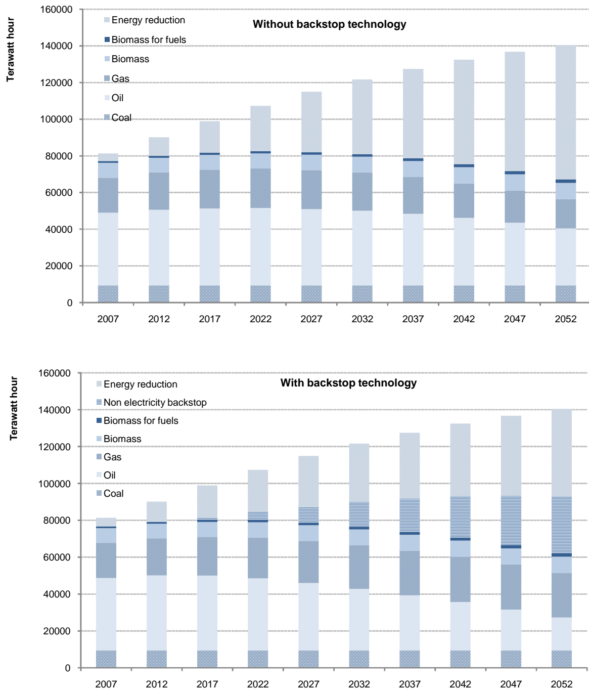
Figure 11. Projected energy technology mix in the non electricity sector under a 550ppm GHG concentration stabilisation scenario, with and without non electricity backstop technology 1
