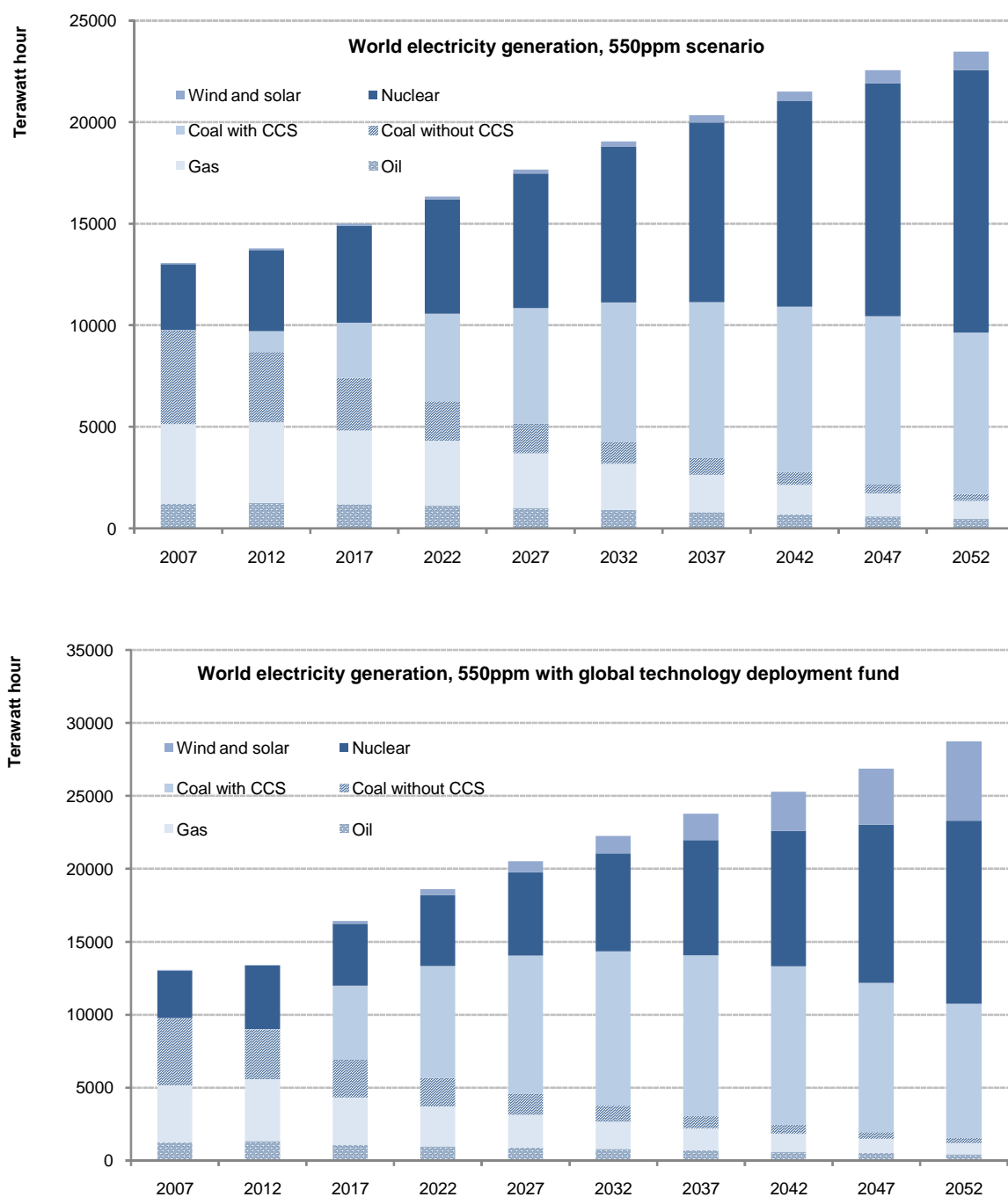
Figure 20. Projected energy technology mix in the electricity sector under a 550ppm GHG concentration stabilisation scenario, with and without a global technology deployment fund 1
