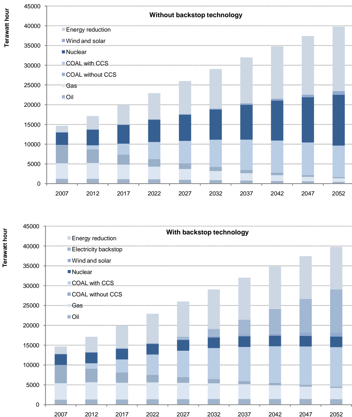
Figure 10. Projected energy technology mix in the electricity sector under a 550ppm GHG concentration stabilisation scenario, with and without electricity backstop technology 1
