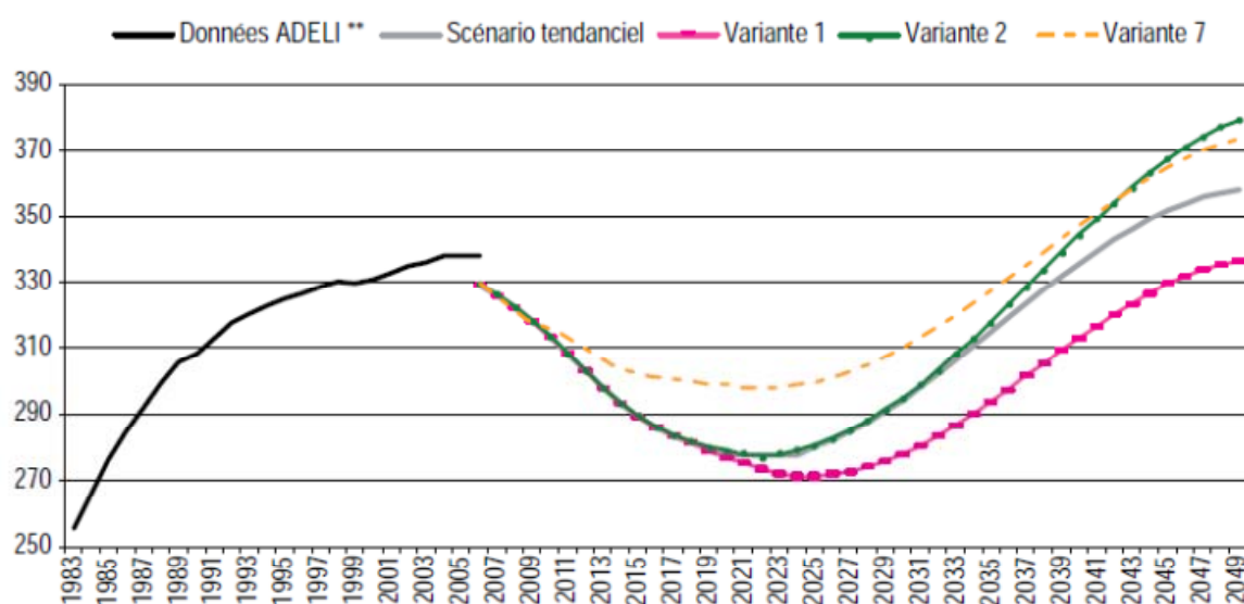
Figure 7. Physician density (per 100,000 population) in France, baseline scenario and scenarios 1, 2, and 7, 2007-2050
