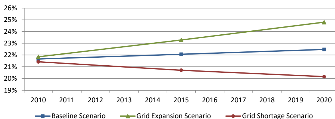
Figure 10. Simulation of average ECF in the European Union under different assumptions of grid quality
