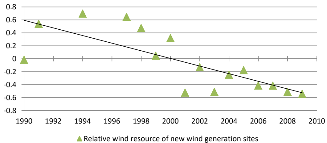
Figure A5. Relative average wind resource of new wind generation sites: Germany
