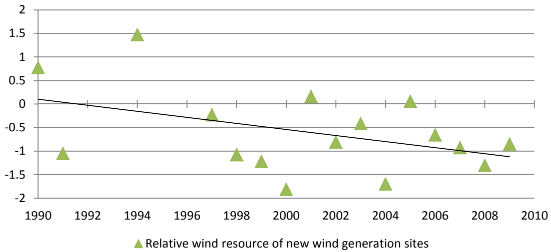
Figure A4. Relative average wind resource of new wind generation sites: Australia
